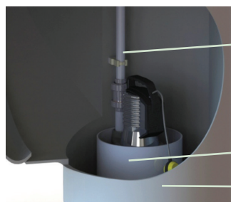
Submersible Pump Option + Tank Internal Pipework & Pump Platform
