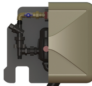
Pre-Assembled RainWorx Cabinet - Wall Mountable
