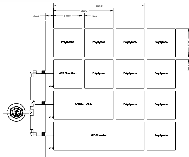
Typical Stormslab layout in "Rib Rati" Style Concrete Floor Layout
