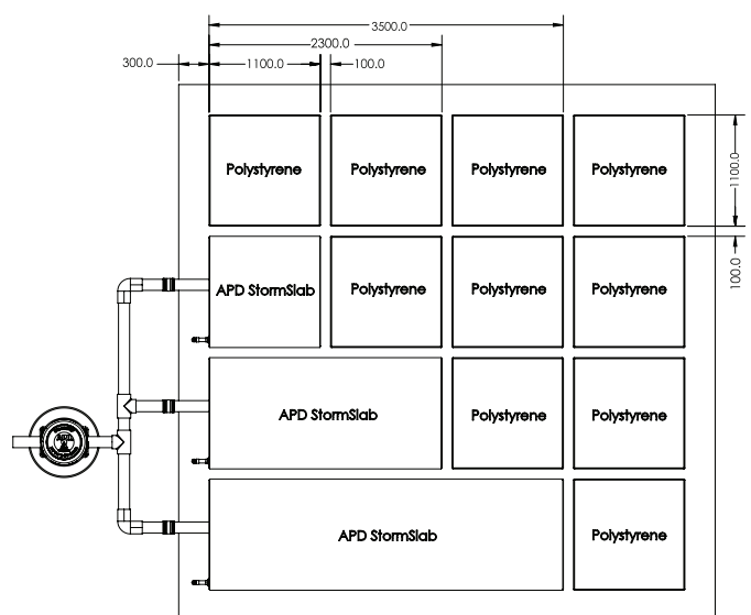
Typical Stormslab layout in "Rib Ralf" Style Concrete Floor Layout
