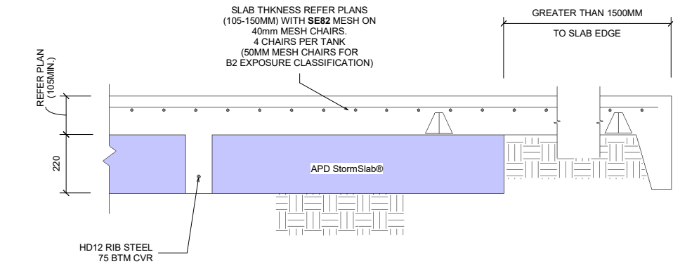
1 DRIVEWAY SLAB - TANKS GREATER THAN 1500MM TO SLAB EDGE
