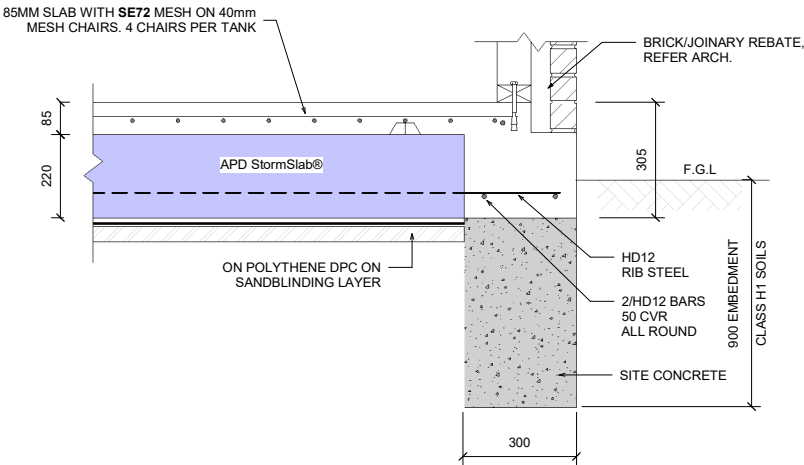
1 TYPICAL SLAB - EDGE RIB WITH SITE CONCRETE.
