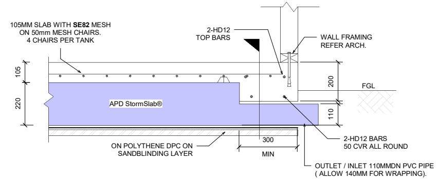
4 GARAGE SLAB - EDGE RIB WITH FLOW THROUGH
