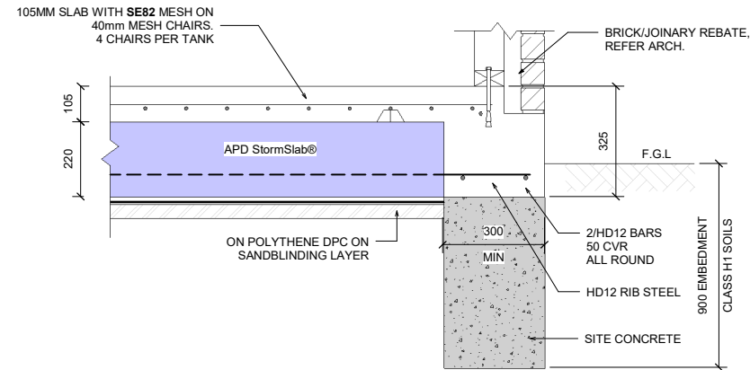
2 GARAGE SLAB - EDGE RIB WITH BRICK REBATE
