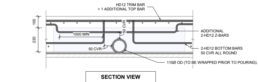
0 TYPICAL SLAB - INTERNAL RIB
