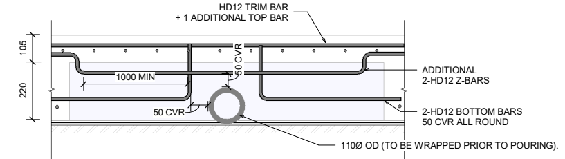
SECTION VIEW
