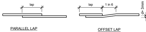
PARALLEL LAP
