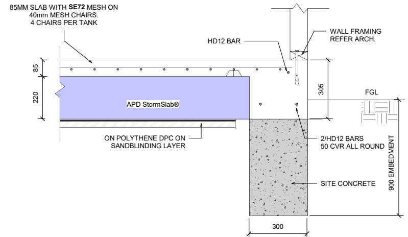
6 TYPICAL SLAB - EDGE RIB WITH SITE CONCRETE
